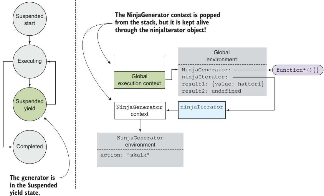
Figure 6.9 After yielding a value, the generator's execution context is popped from the stack (but isn't discarded, because ninjaIterator keeps a reference to it), and the generator execution is suspended (the generator moves to the Suspended yield state).
