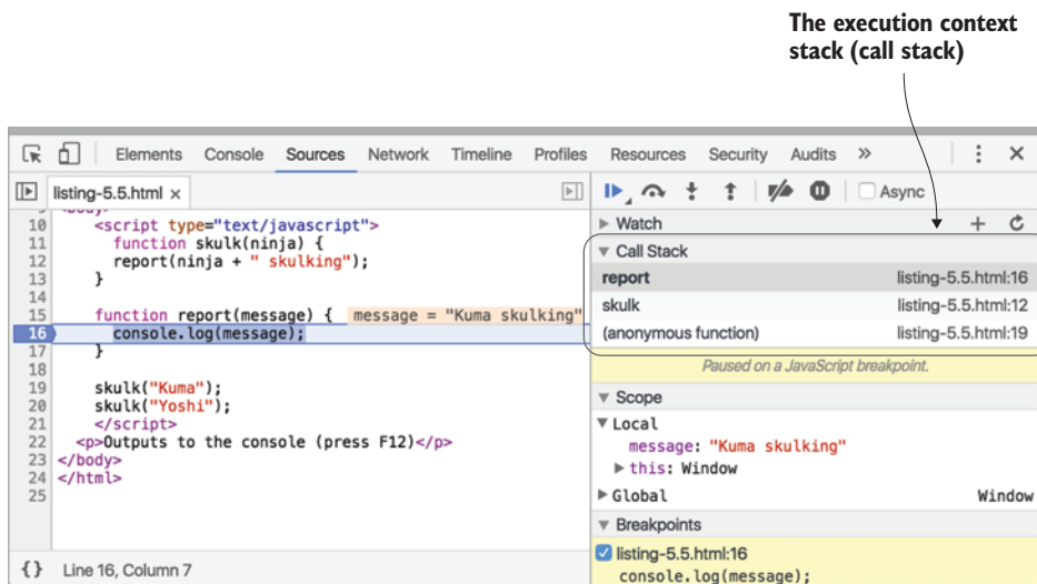
Figure 5.7 The current state of the execution context stack in Chrome DevTools
